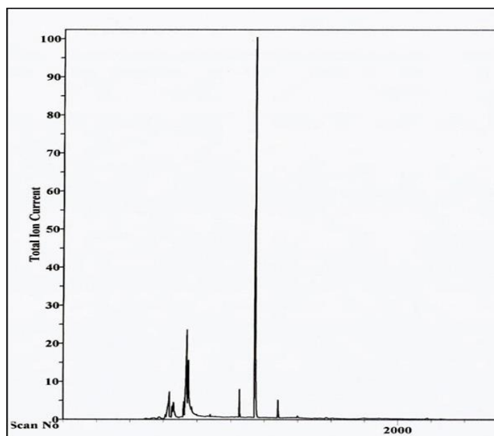
Figure 2: The GCMS chromatogram of A. terreus MP15 fungal ethyl acetate extract
