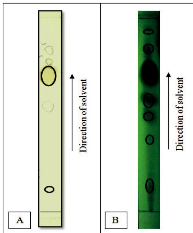
Figure 1: TLC chromatograms of fungal isolate A. terreus MP15 crude ethyl acetate extract viewed under (A) visible light and (B) short wavelength with solvent system dichloromethane: methanol at ratio 9:1
